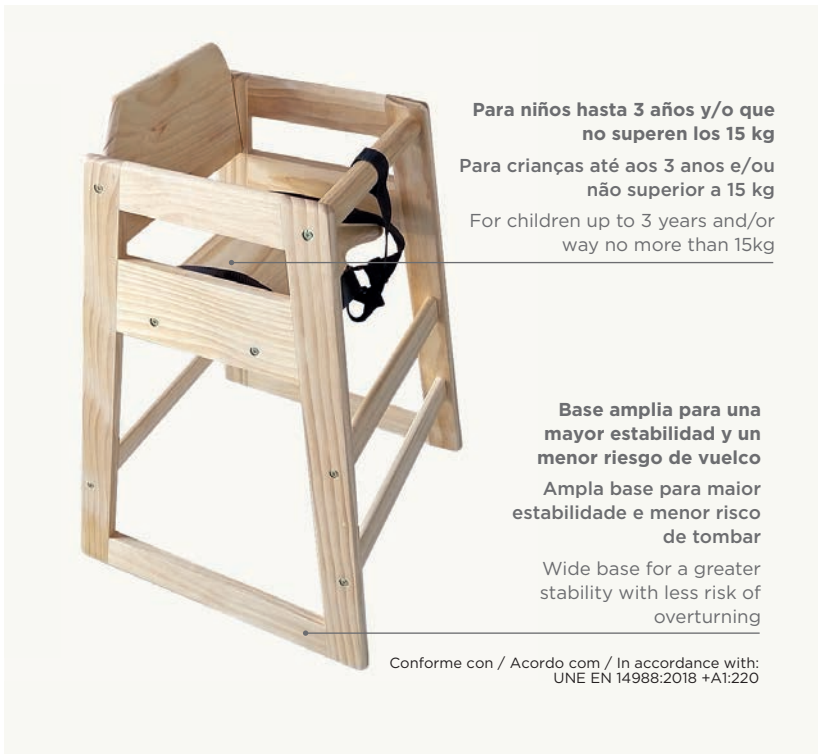
133.98 30 x 30 x 28 cm Madera nogal Madeira nogueira Walnut wood PACK / MINIM: 1 U
